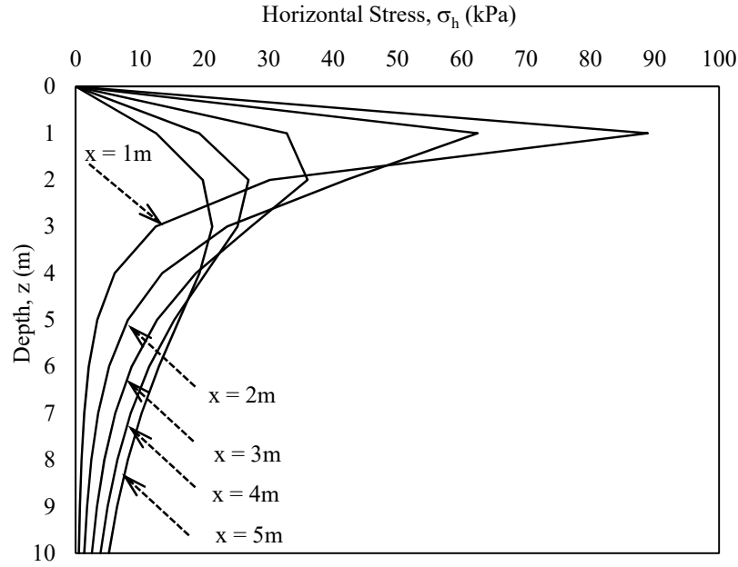
Fig. 5: Horizontal Stress Variation with Depth for Strip Load Width, B = 2.5\text{m}
