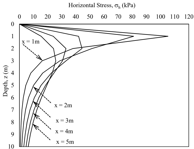
Fig. 6: Horizontal Stress Variation with Depth for Strip Load Width, B = 3\text{m}
